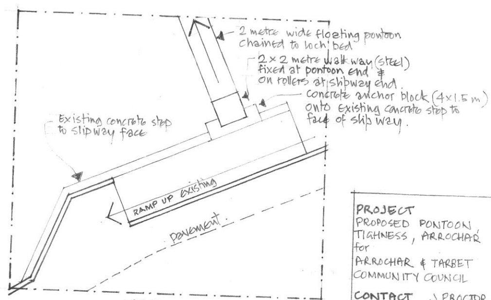
PLAN C PONTOON/SLIP INTERFACE - DO ANCHOR
